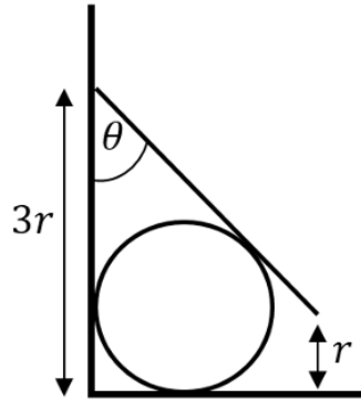
Figure 4: A hinged rod resting on a cylinder.
